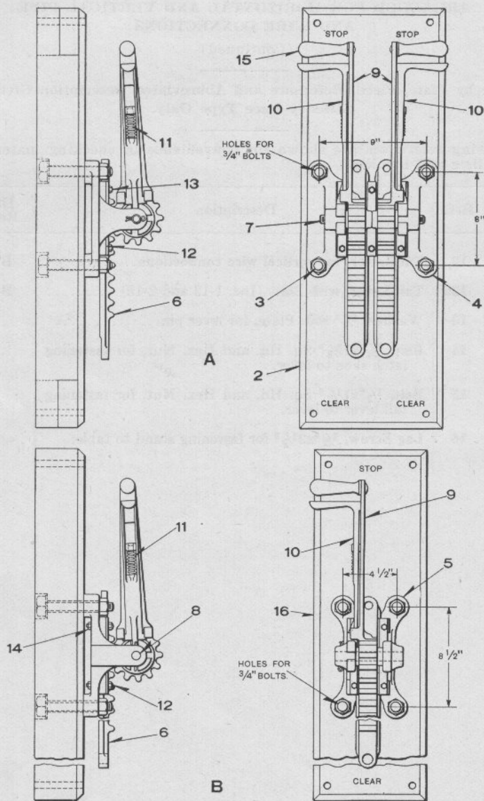
1 AND 2 LEVER, 2 AND 3 POSITIONS, A. R. A. WALL MACHINES
